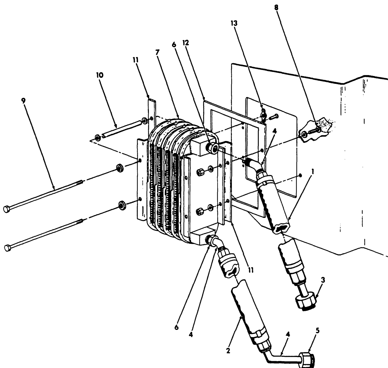
Lube Oil Cooler Installation Figure 79-2
