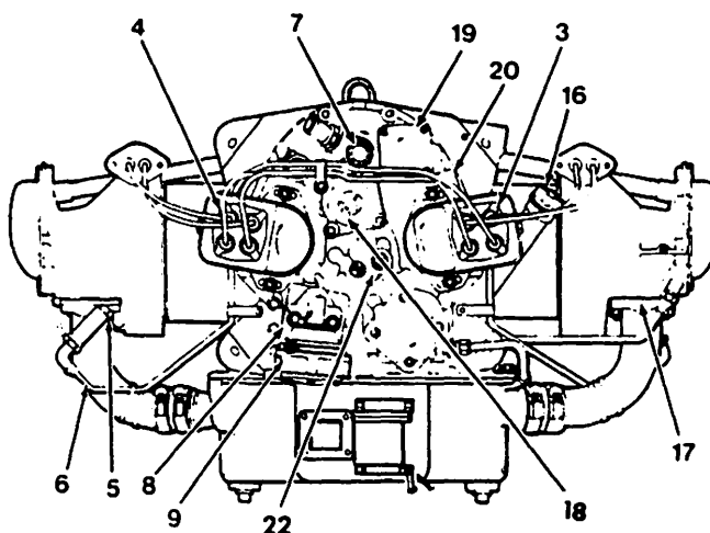
Engine and Accessories Installation Figure 71-1
