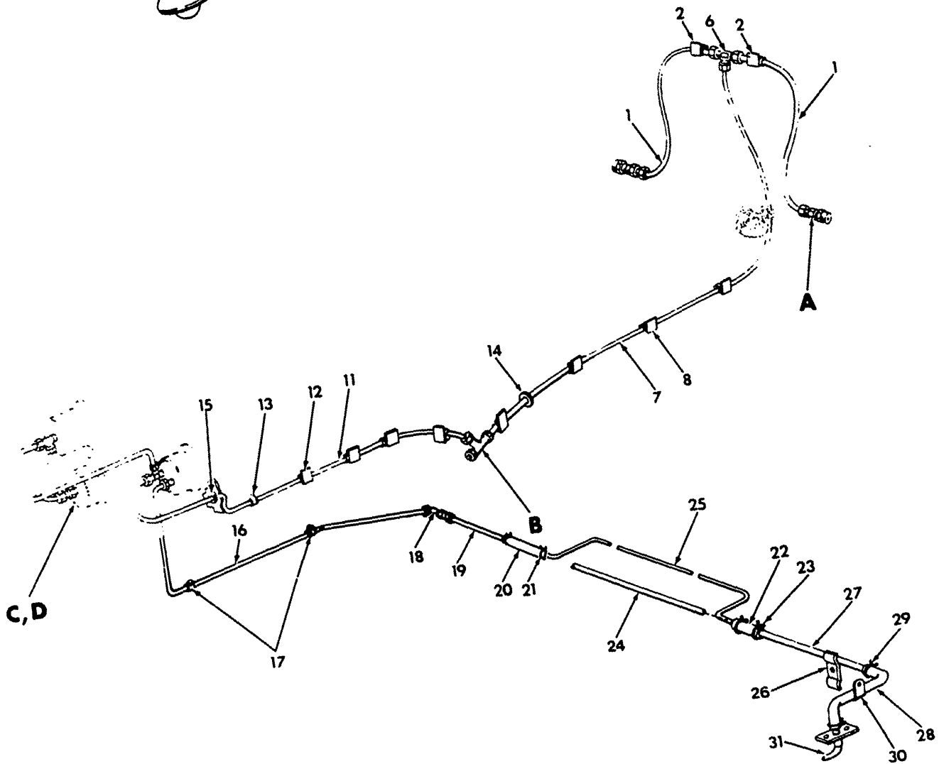
Airspeed System Installation (Sheet 1 of 2) Figure 34-3
