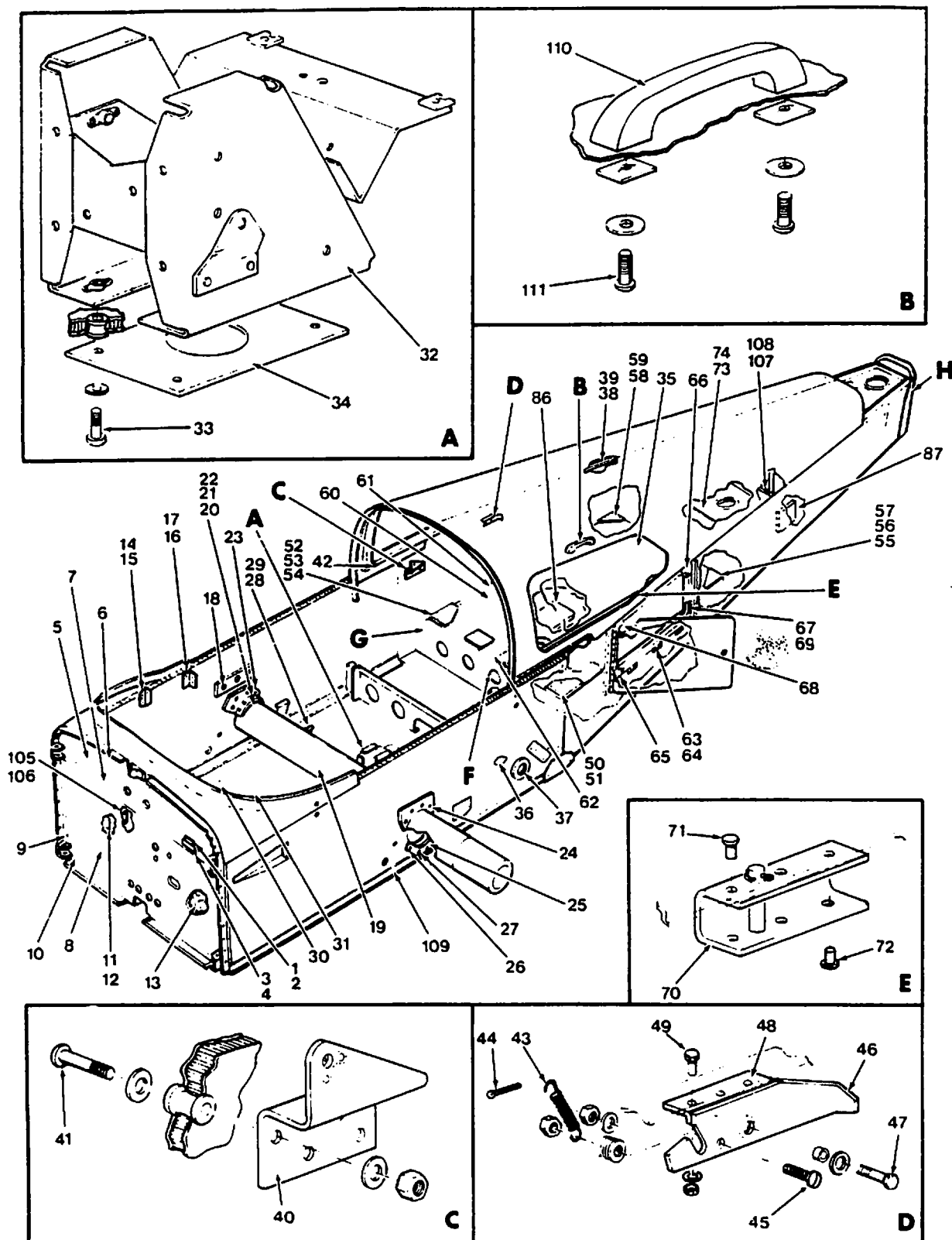
Fuselage Assembly (Sheet 1 of 2) Figure 53-1
