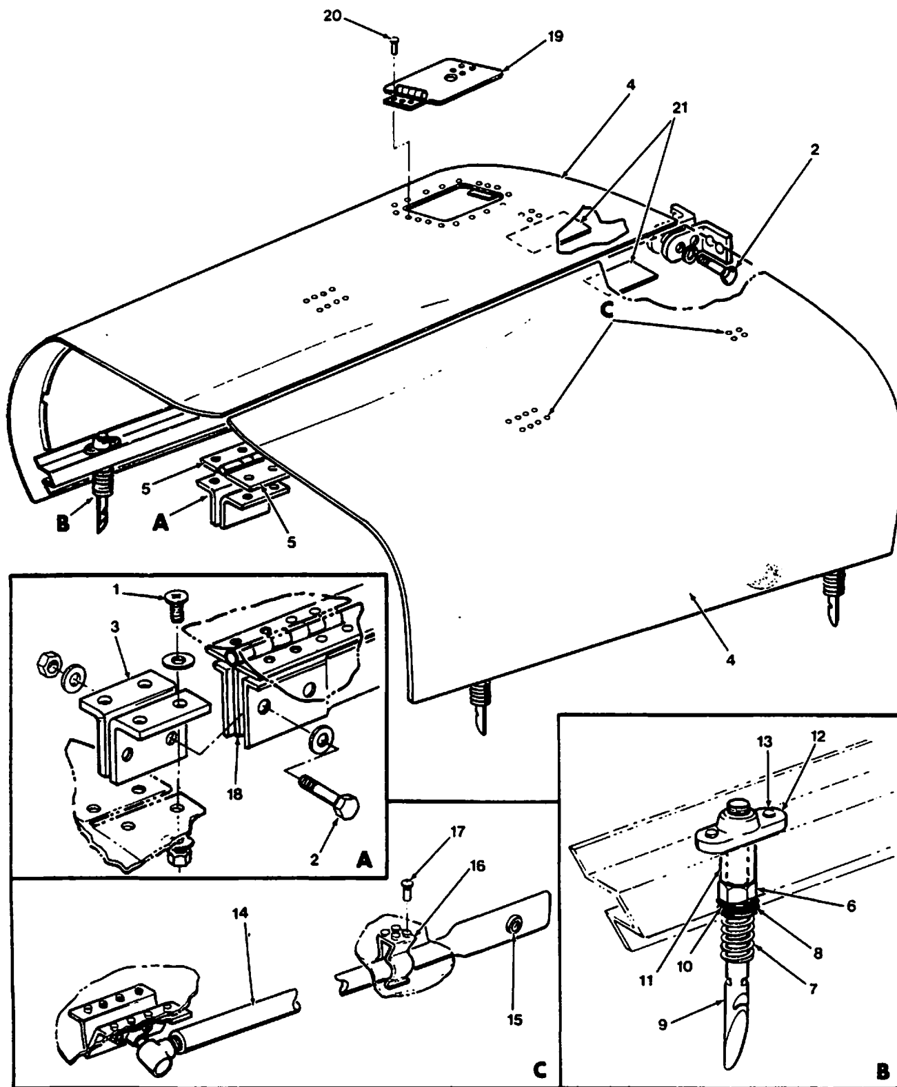
Upper Cowl Installation Figure 71-5
