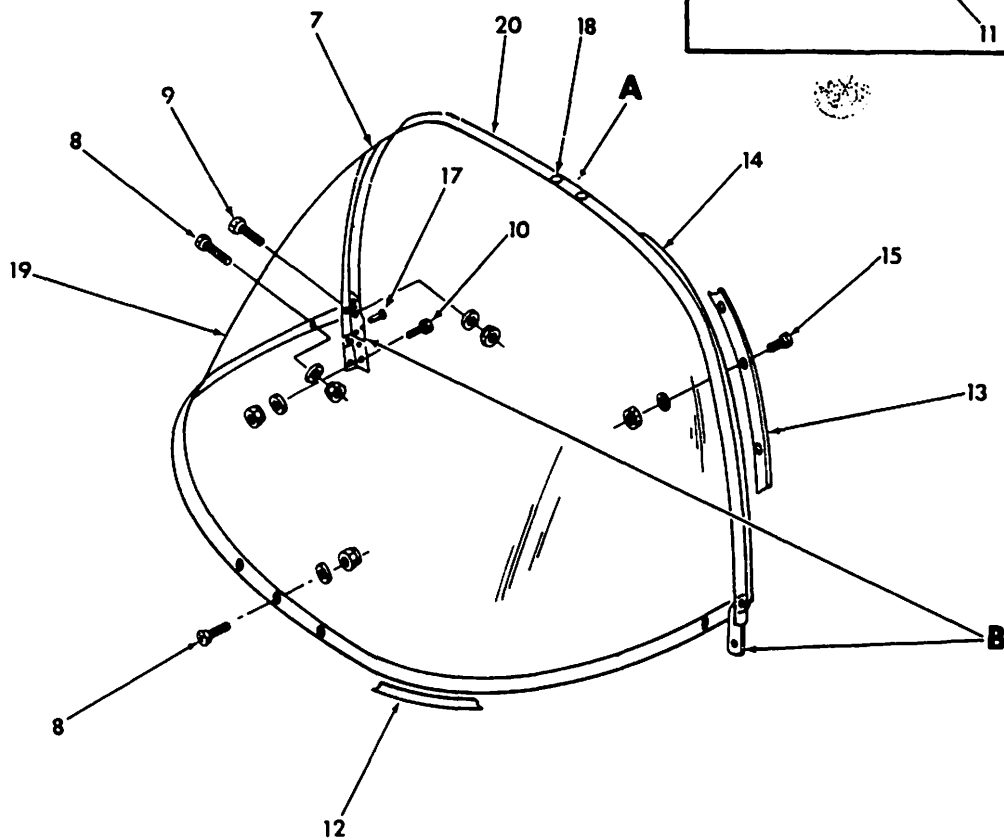
Windshield Installation Figure 56-1
