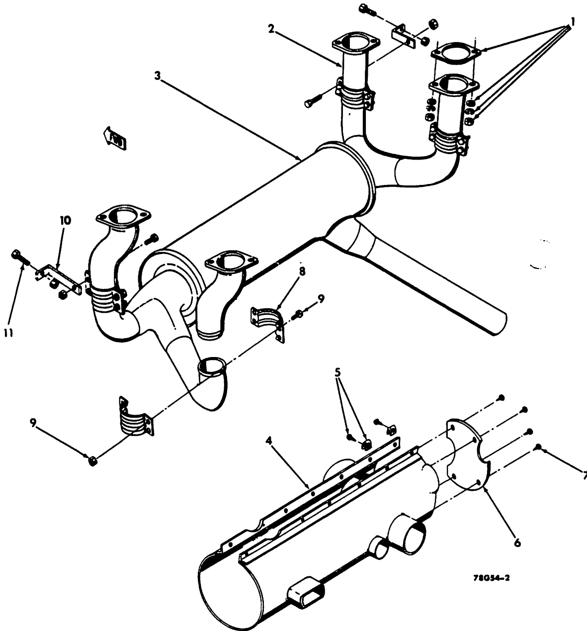
Heater - Muffler Exhaust Installation (AA-5B) Figure 78-2
