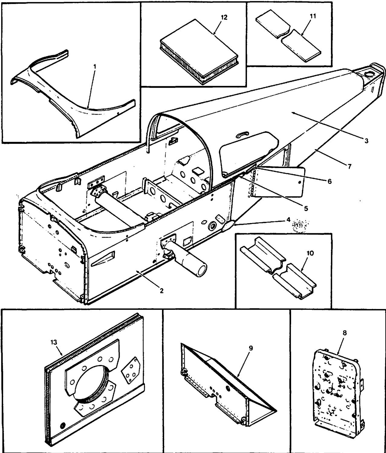
Fuselage Assembly (Spares) Figure 53-3
