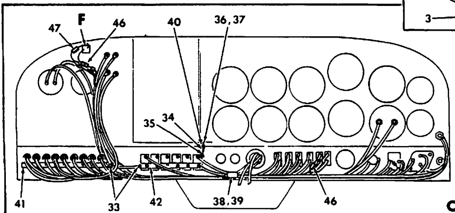
Electrical System Installation Figure 24-1 (Sheet 1 of 2)
