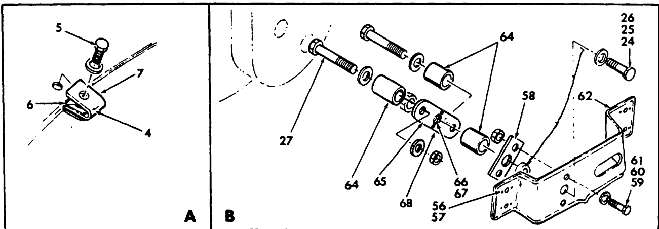
Main Landing Gear Fairing Installation Figure 32-7
