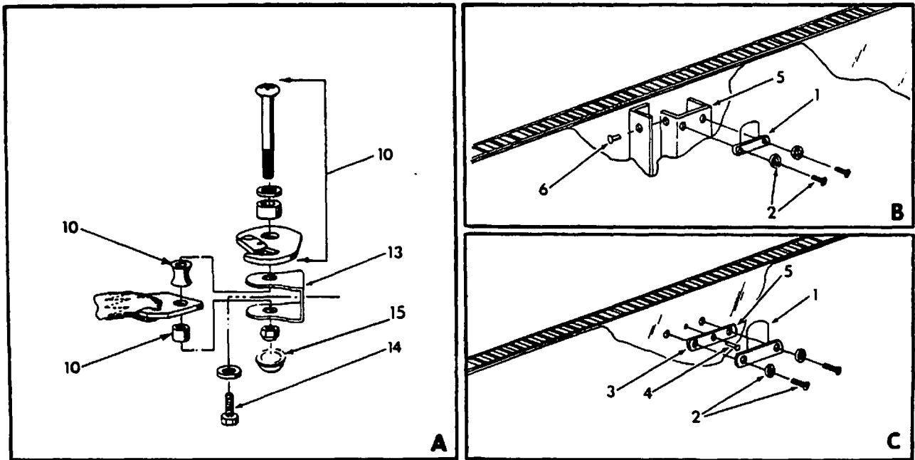
Belt Installation Figure 25-1
