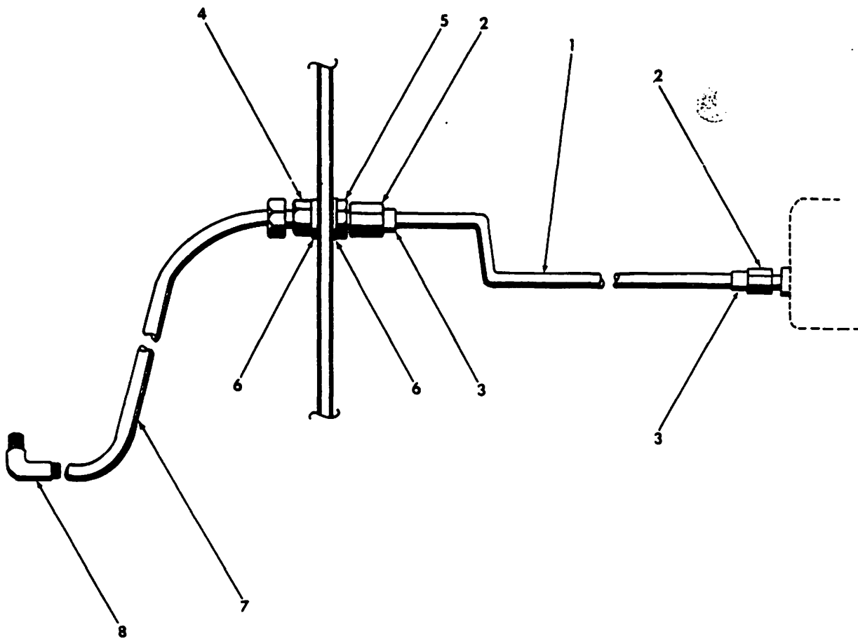
Oil Pressure Line Figure 79-1
