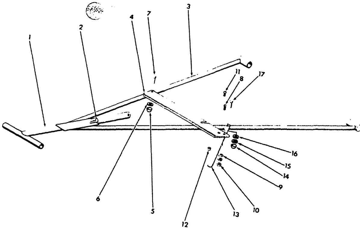
Tow Bar Assembly Figure 12-1
