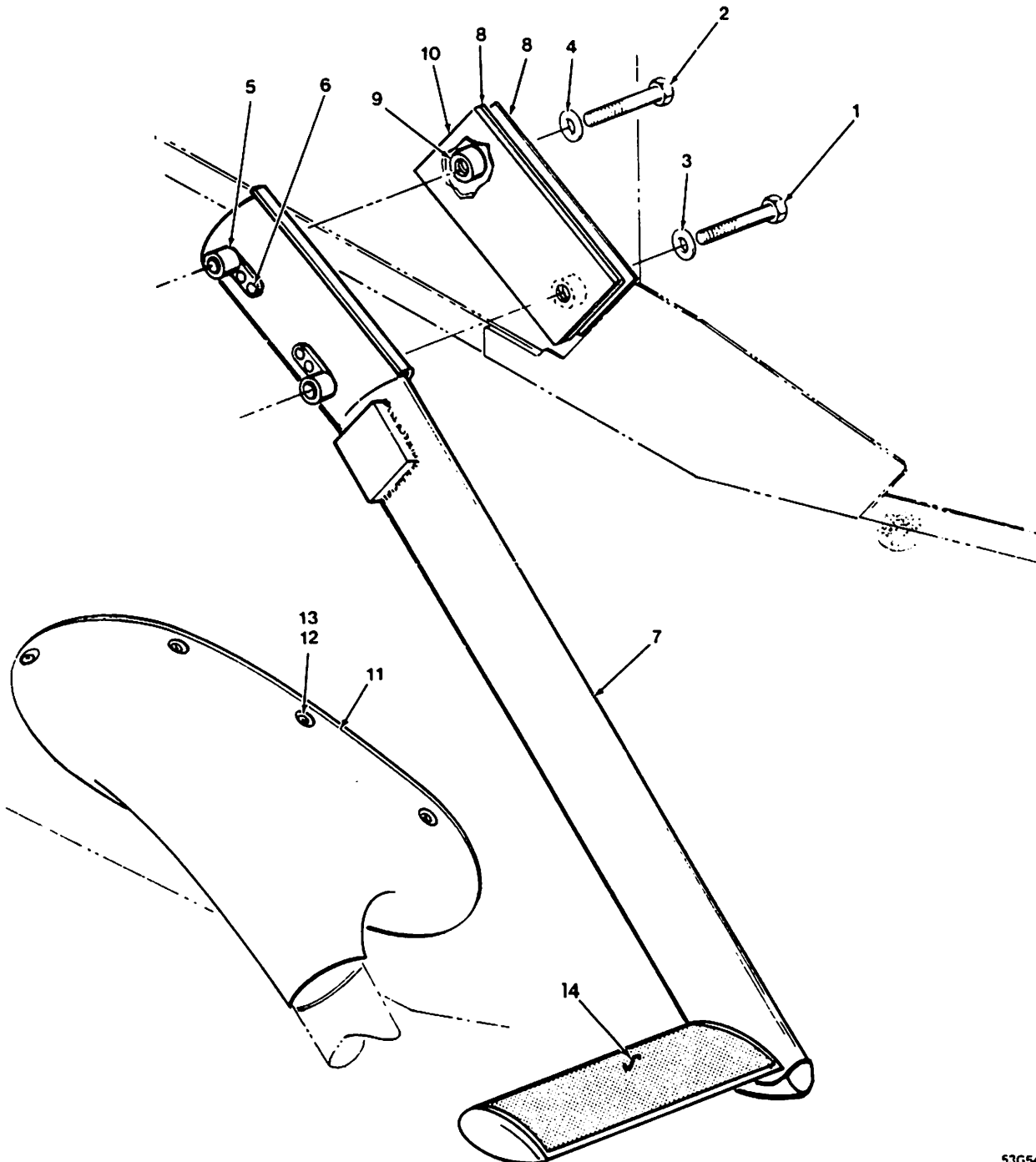
Passenger Step Installation (Optional) Figure 53-5
