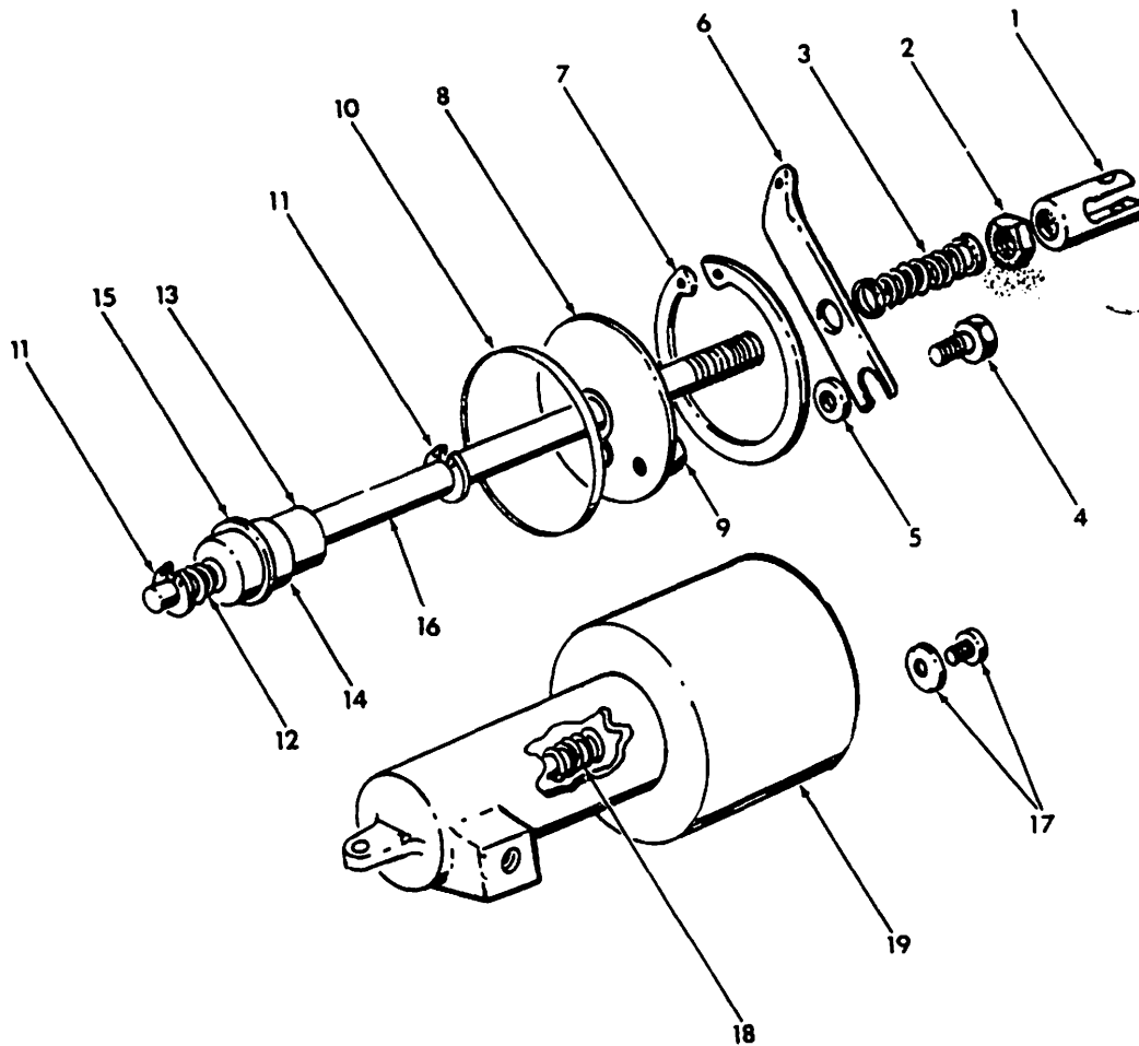
Master Cylinder Figure 32-13
