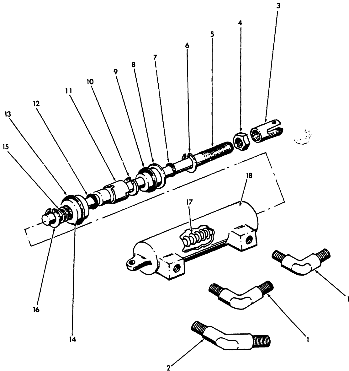
Master Cylinder Assembly Figure 32-14
