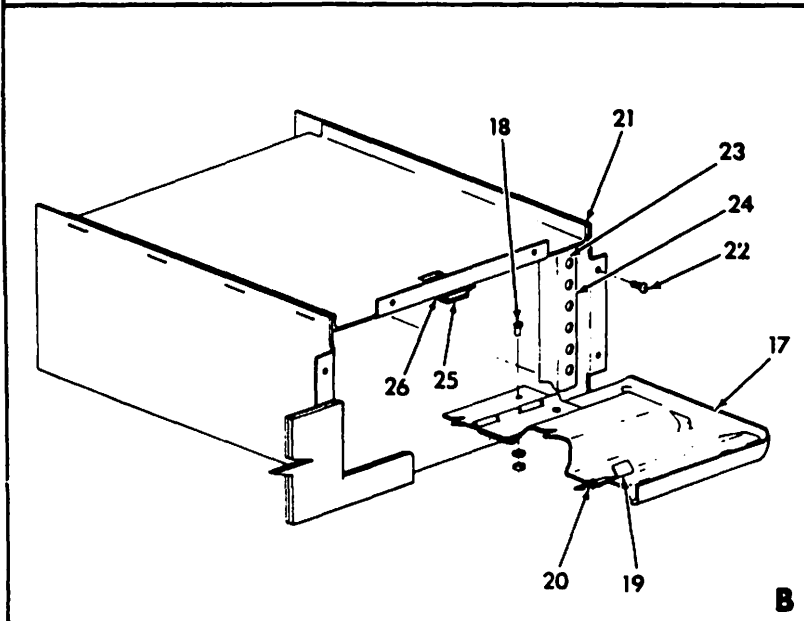
Instrument Panel Installation Figure 34-5
