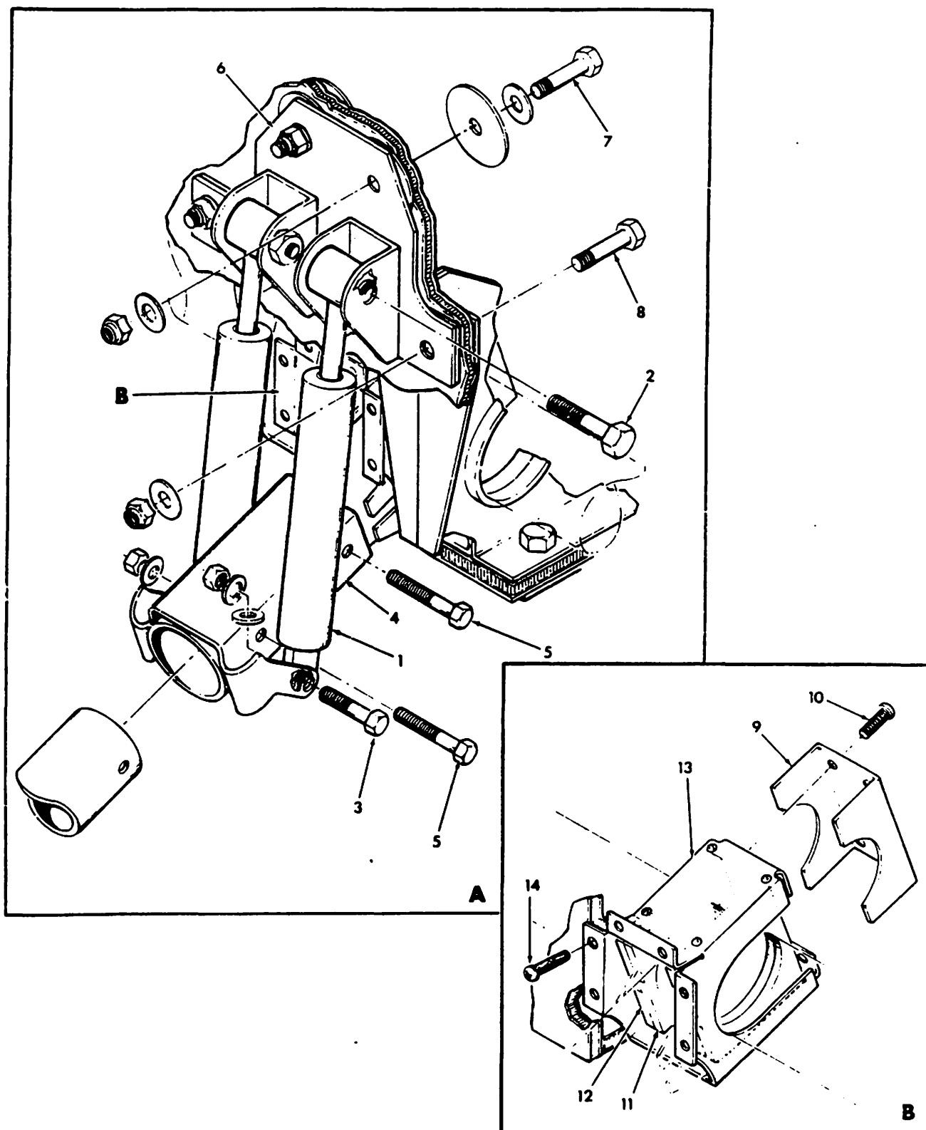
Nose Landing Gear Installation Figure 32-4 (Sheet 2 of 2)
