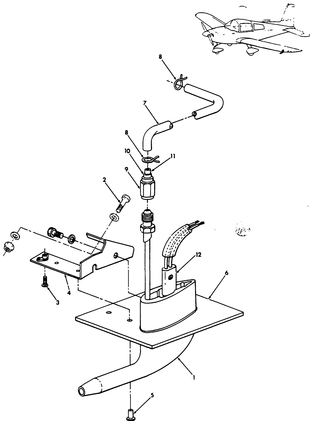
Heated Pitot Tube Installation (Optional) Figure 30-4
