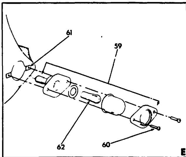
Exterior Light Installations Figure 33-1 (Sheet 2 of 2)
