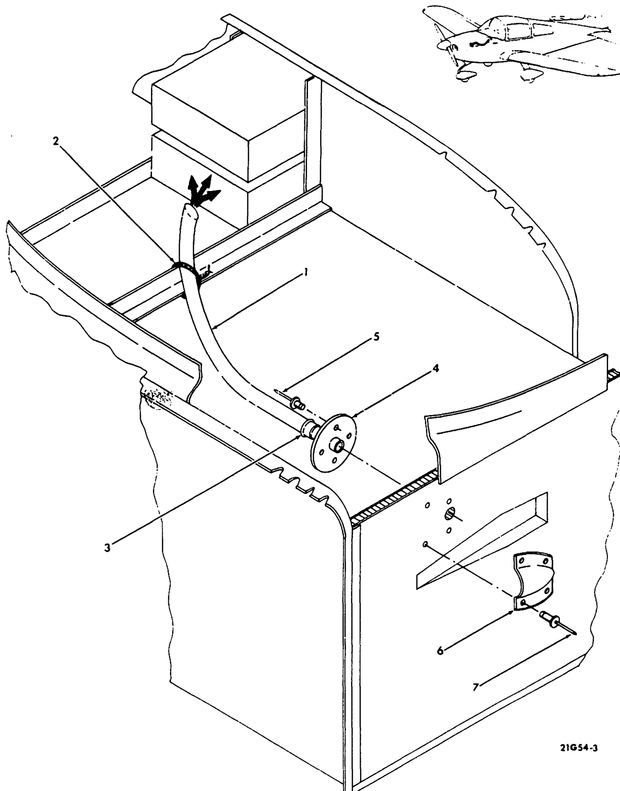
Radio and DME Cooling Kit Installation Figure 21-3
