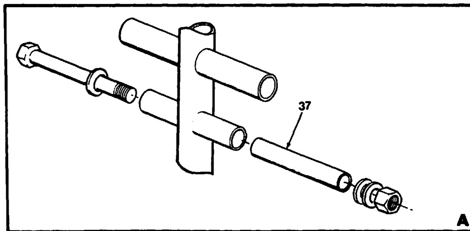
Elevator and Aileron Control Installation Figure 27-1 (Sheet 1 of 3)
