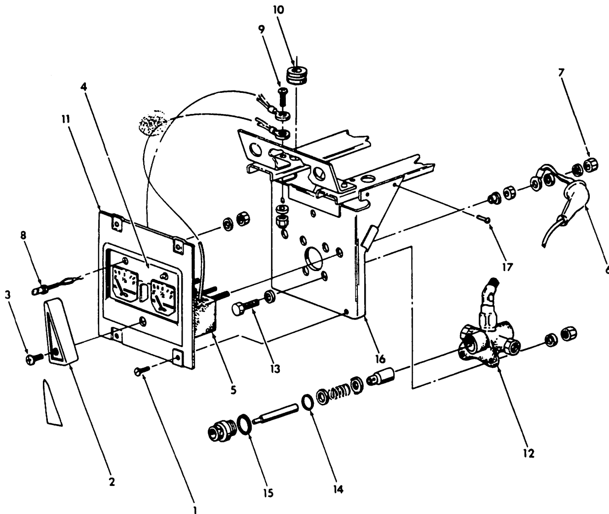
Fuel Valve and Gage Installation Figure 28-2
