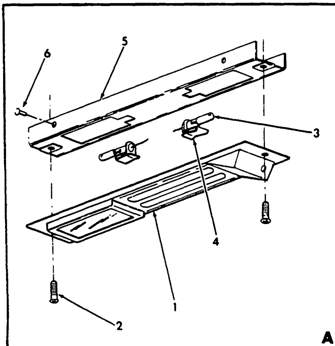
Interior Light Installations Figure 33-2 (Sheet 1 of 2)
