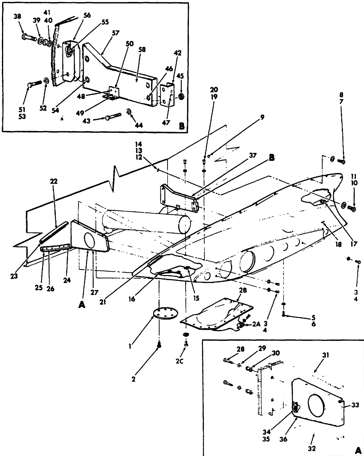
Wing Root Installation Figure 57-3.
