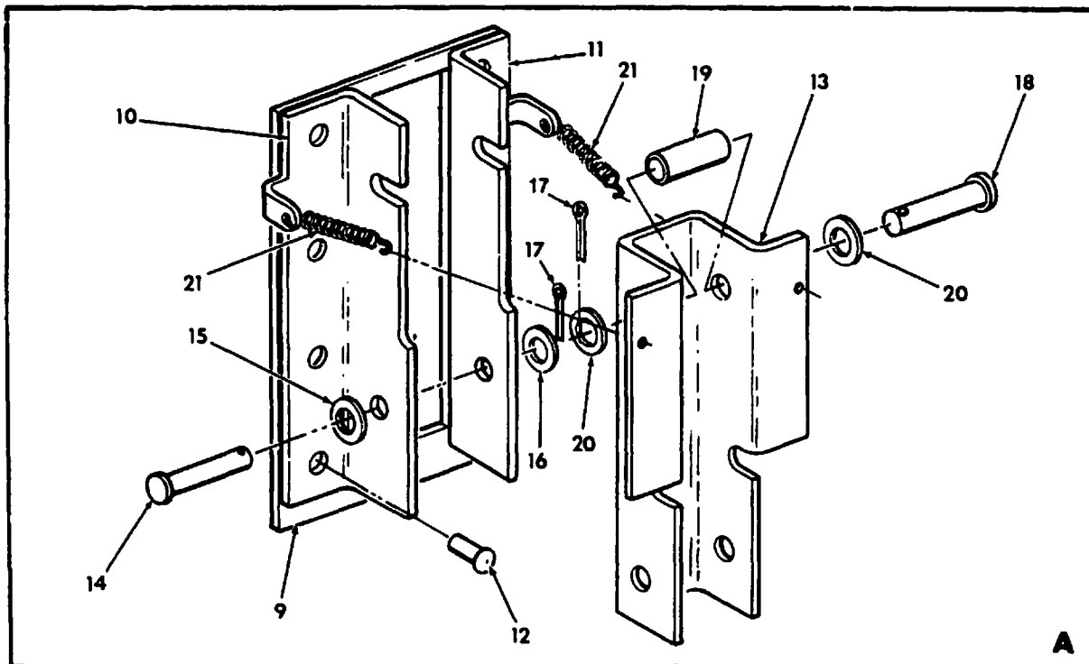
Lower Cowl Installation Figure 71-6
