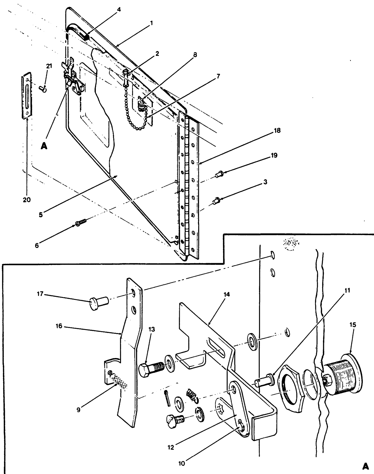
Baggage Door Installation Figure 52-2
