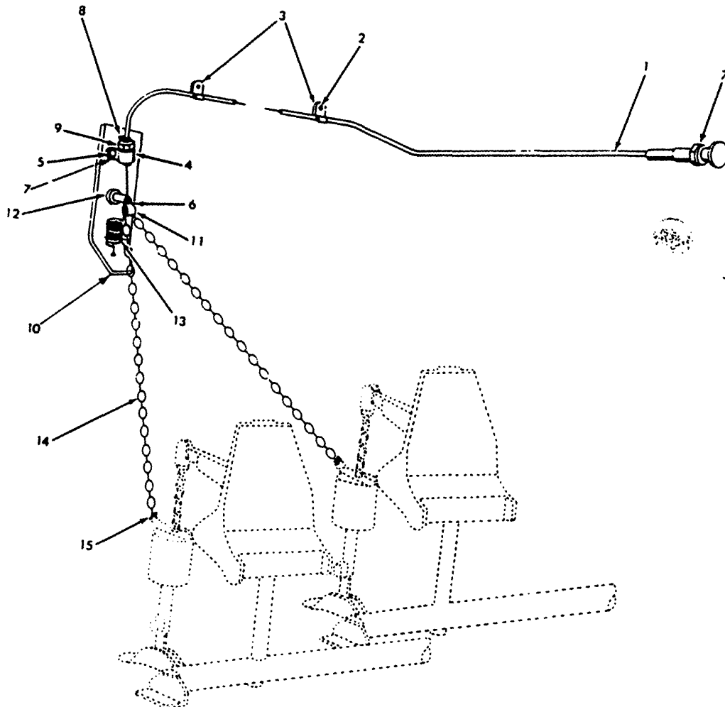
Parking Brake Installation (1977 Models) Figure 32-12
