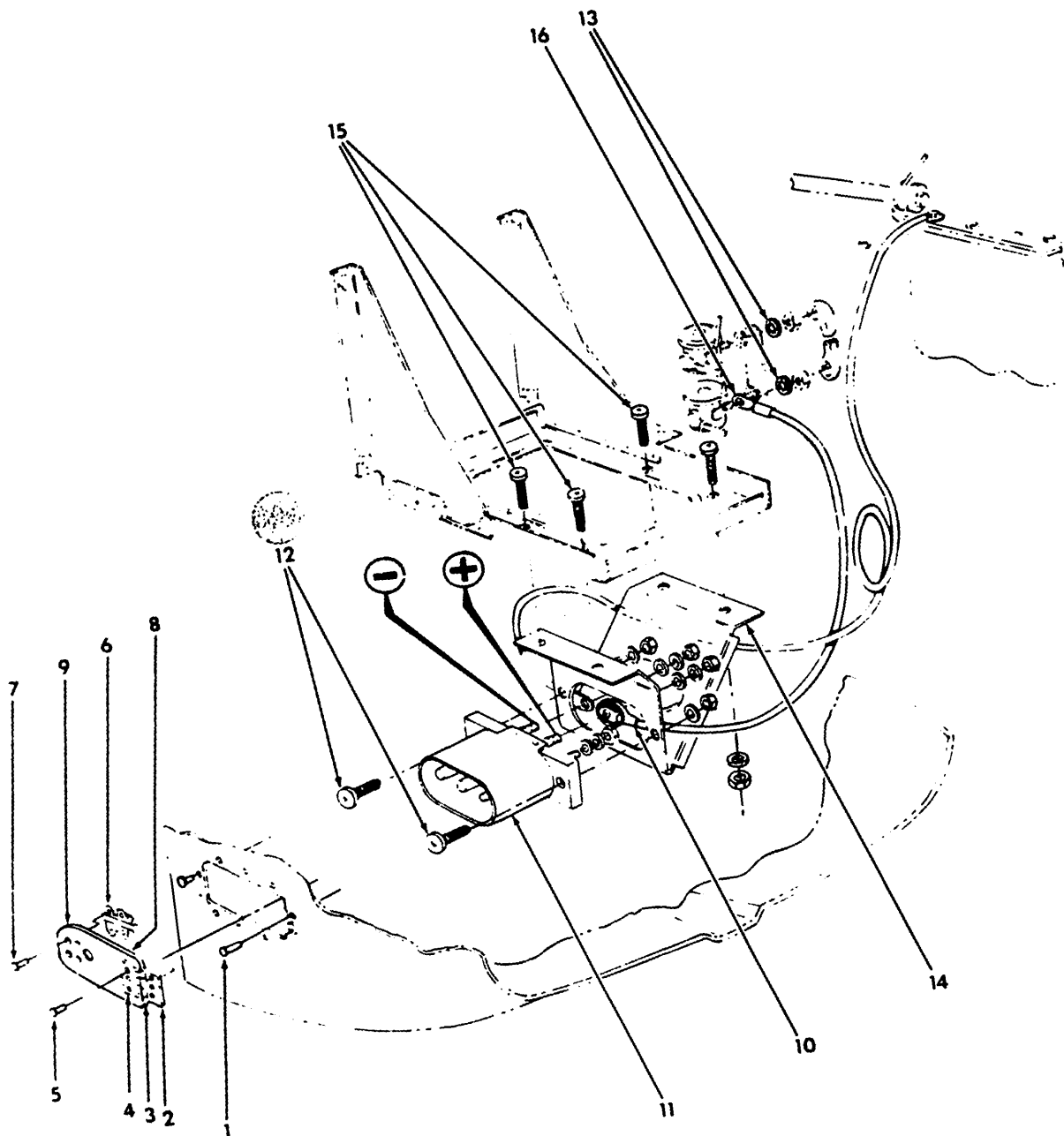
Auxiliary Power Plug Installation (Optional) Figure 24-3
