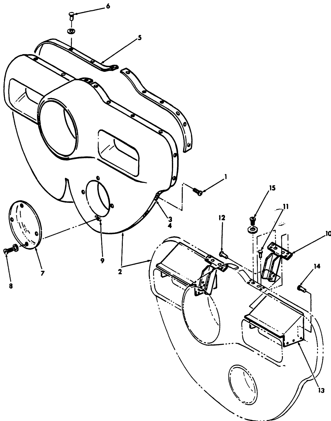
Forward Cowl Installation Figure 71-7
