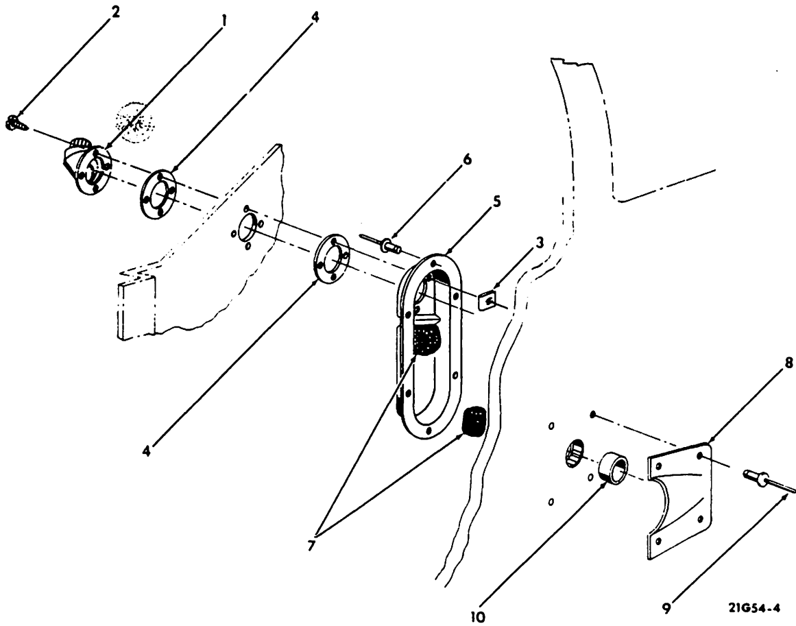
Rear Passenger Vent Installation Figure 21-4
