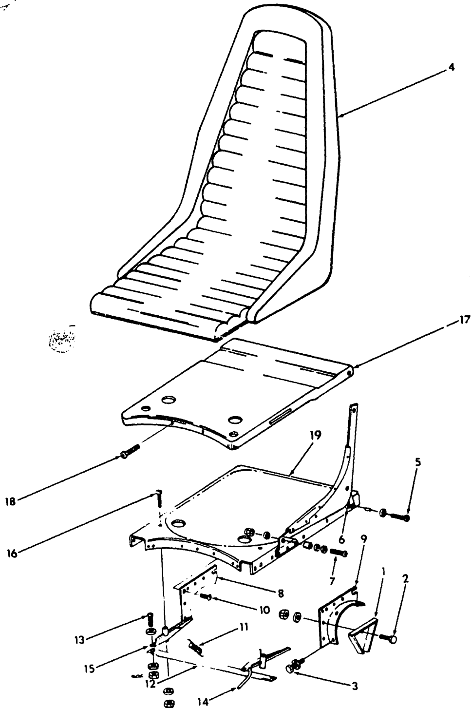
Front Seat Installation (1977 Models) Figure 25-2
