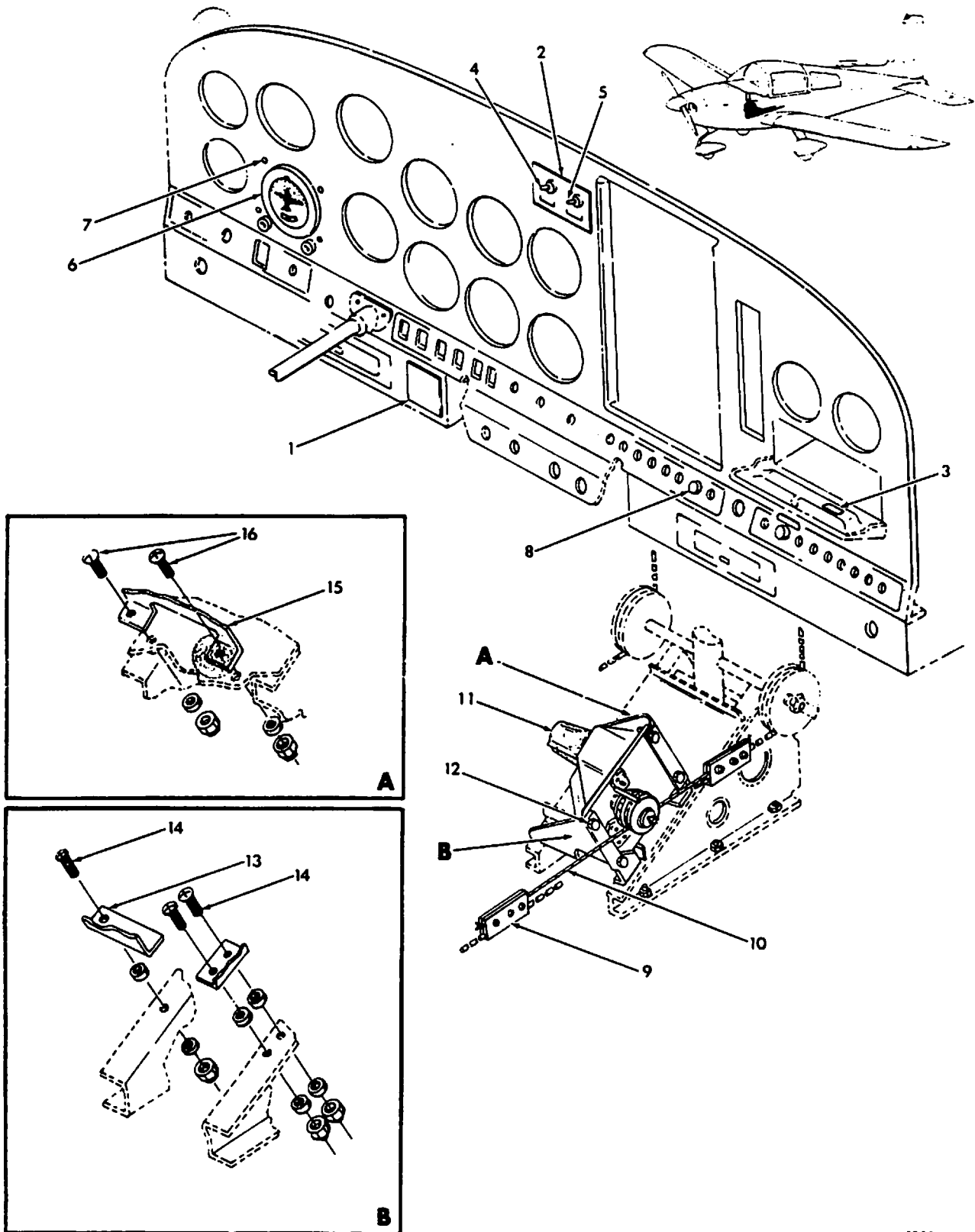
Auto-Pilot Installation - Century I (Optional) Figure 22-1
