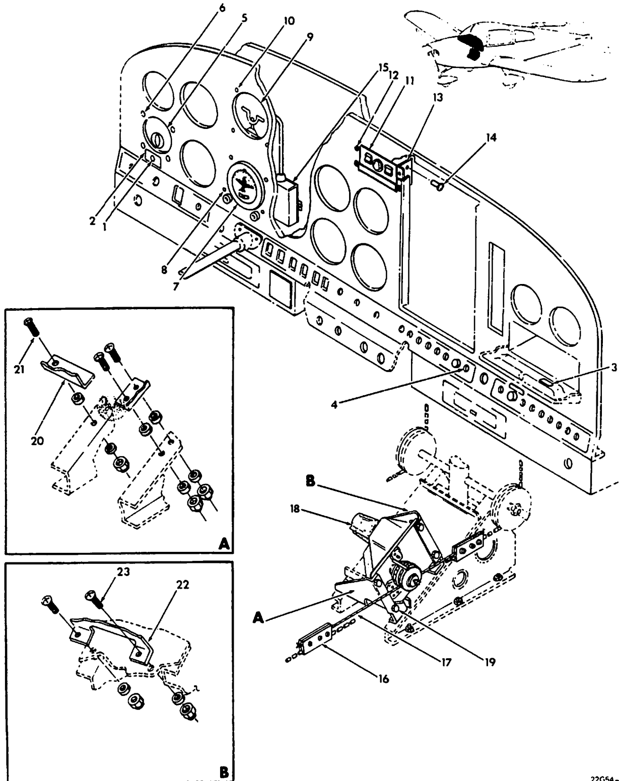
Auto-Pilot Installation — Century II B (Optional) Figure 22-2
